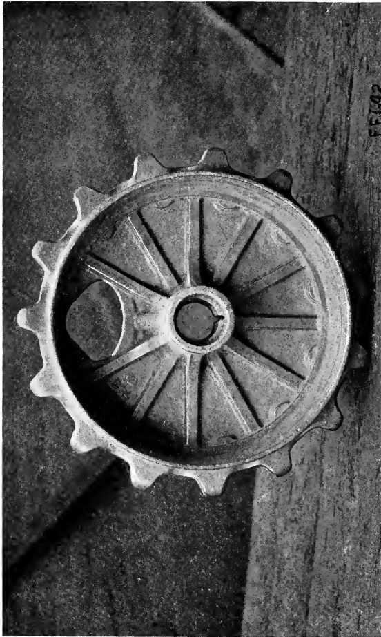
Fig. 40. Upper View—The day's production in Semi-steel.
